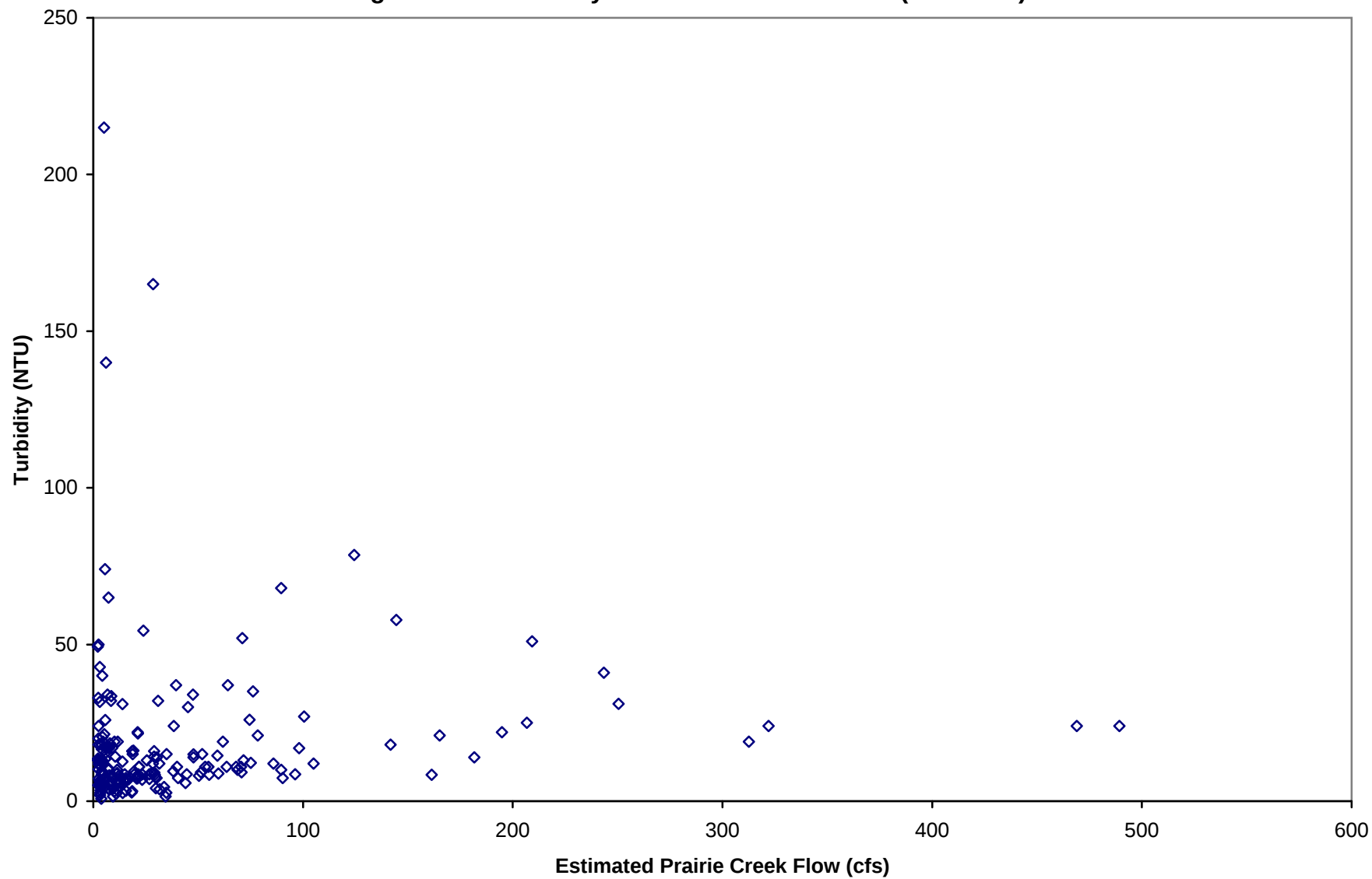
Figure C.19. Turbidity vs Flow in Prairie Creek (OUA0040)
