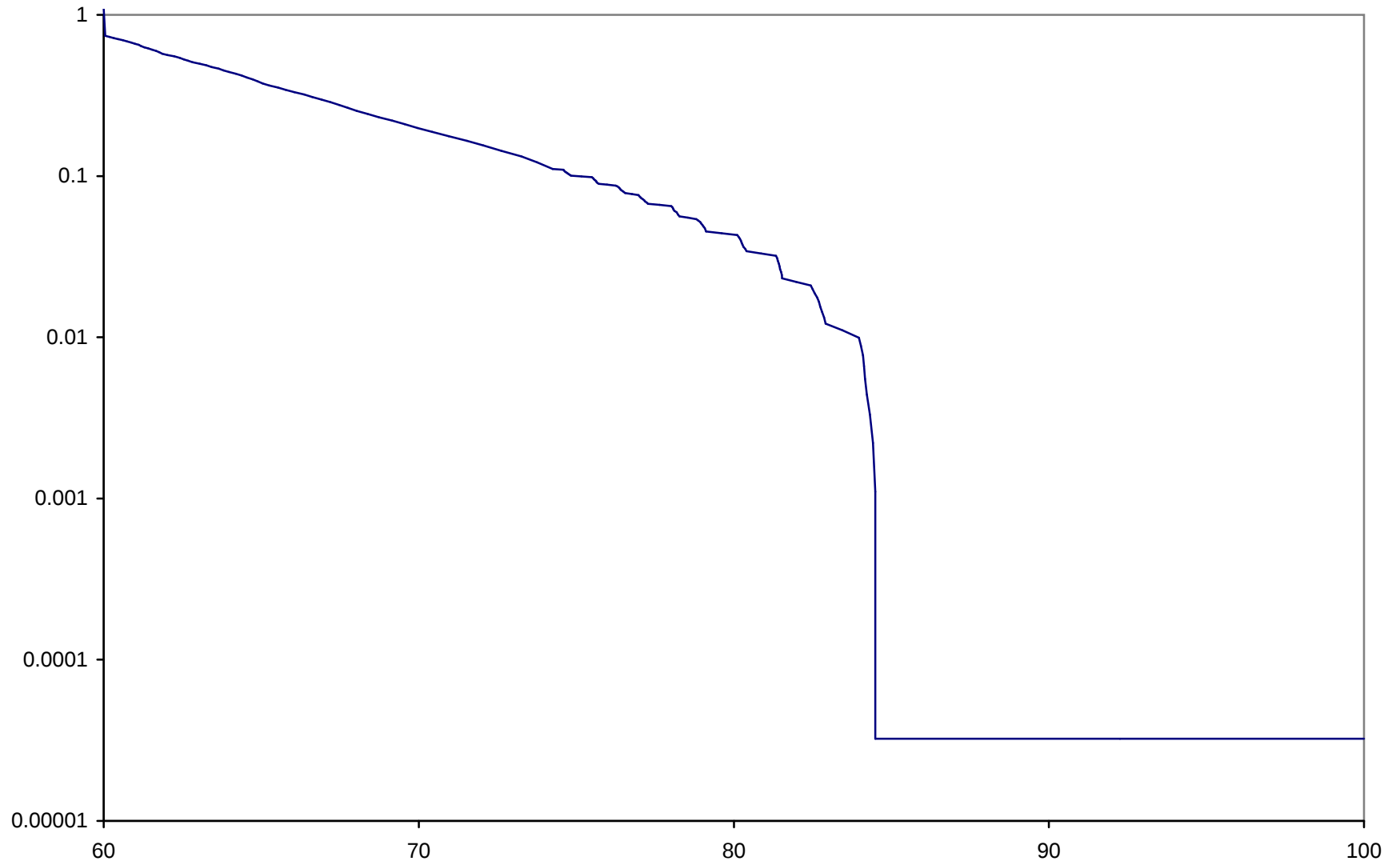
Figure I.3. Base flow load duration curve for Moro Creek (08040201-001L)
