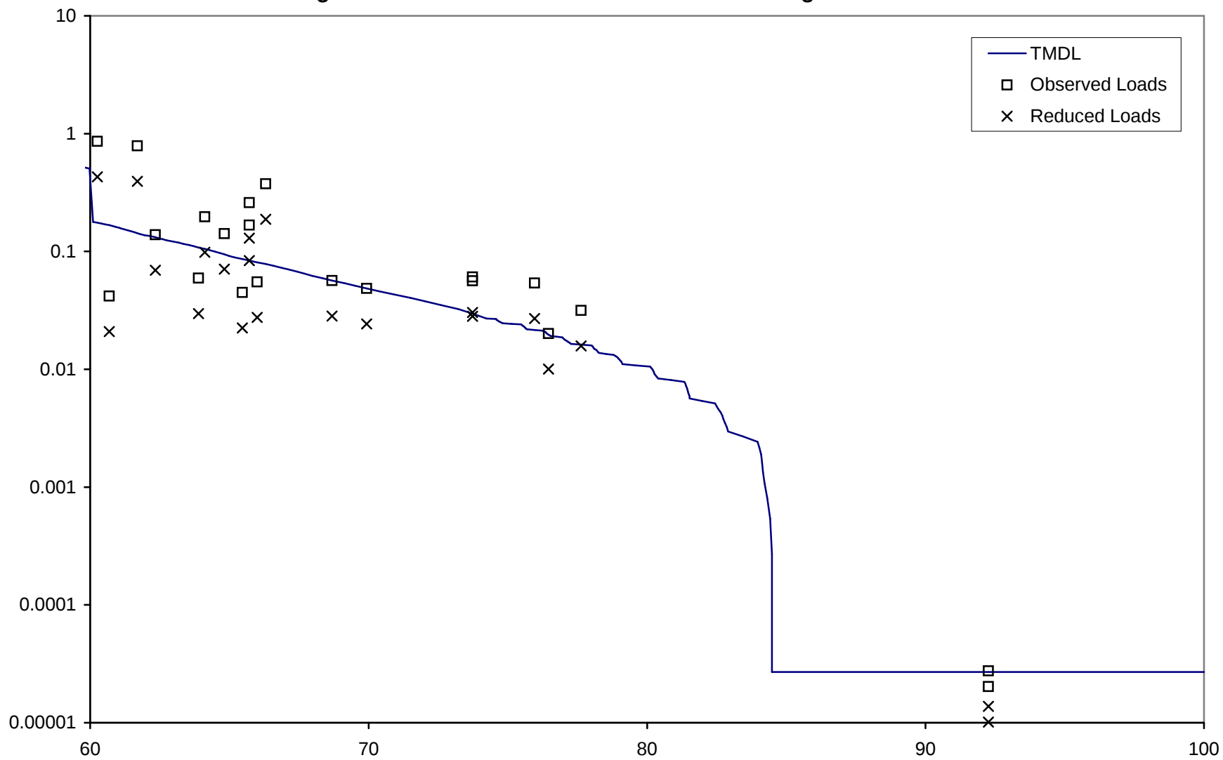
Figure J.3. Base flow load duration curve for Big Creek
