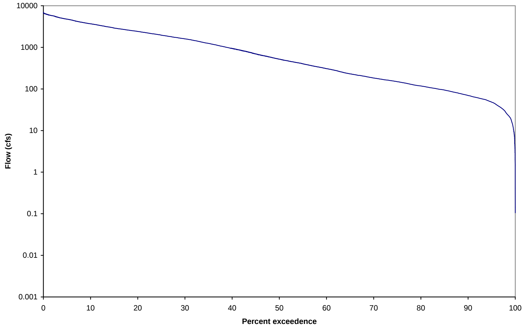
Figure H.1. Flow duration curve for Bayou Bartholomew reach 08040205-002
