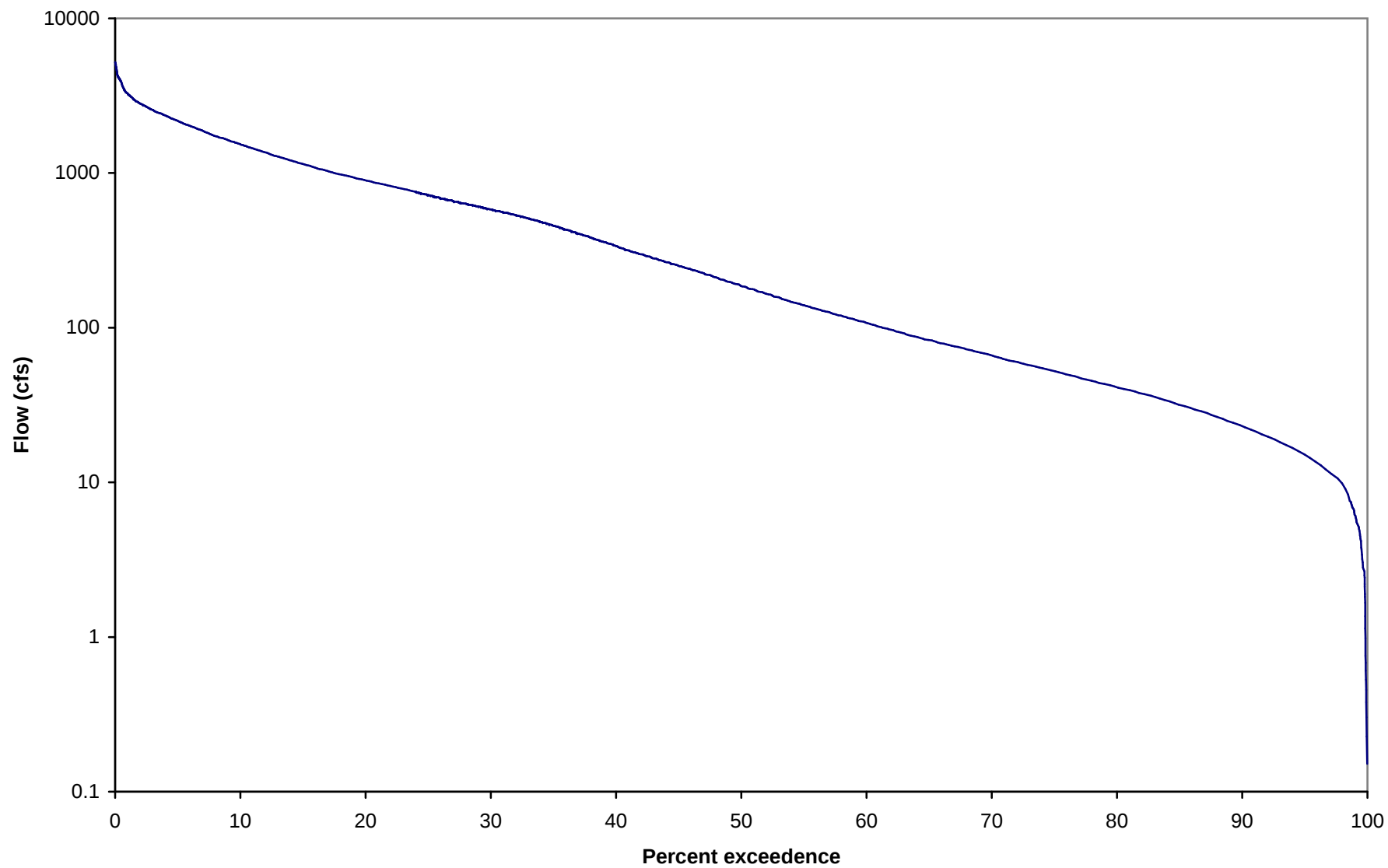
Figure F.1. Flow duration curve for Bayou Bartholomew reach 08040205-013
