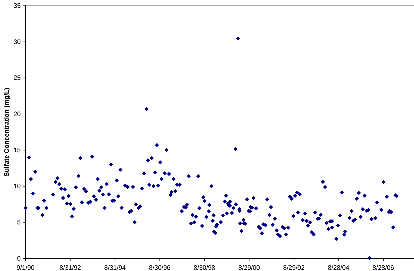
Figure B.11. Time Series Plot of Sulfate in Bayou Bartholomew near Jones, LA (OUA0013)
