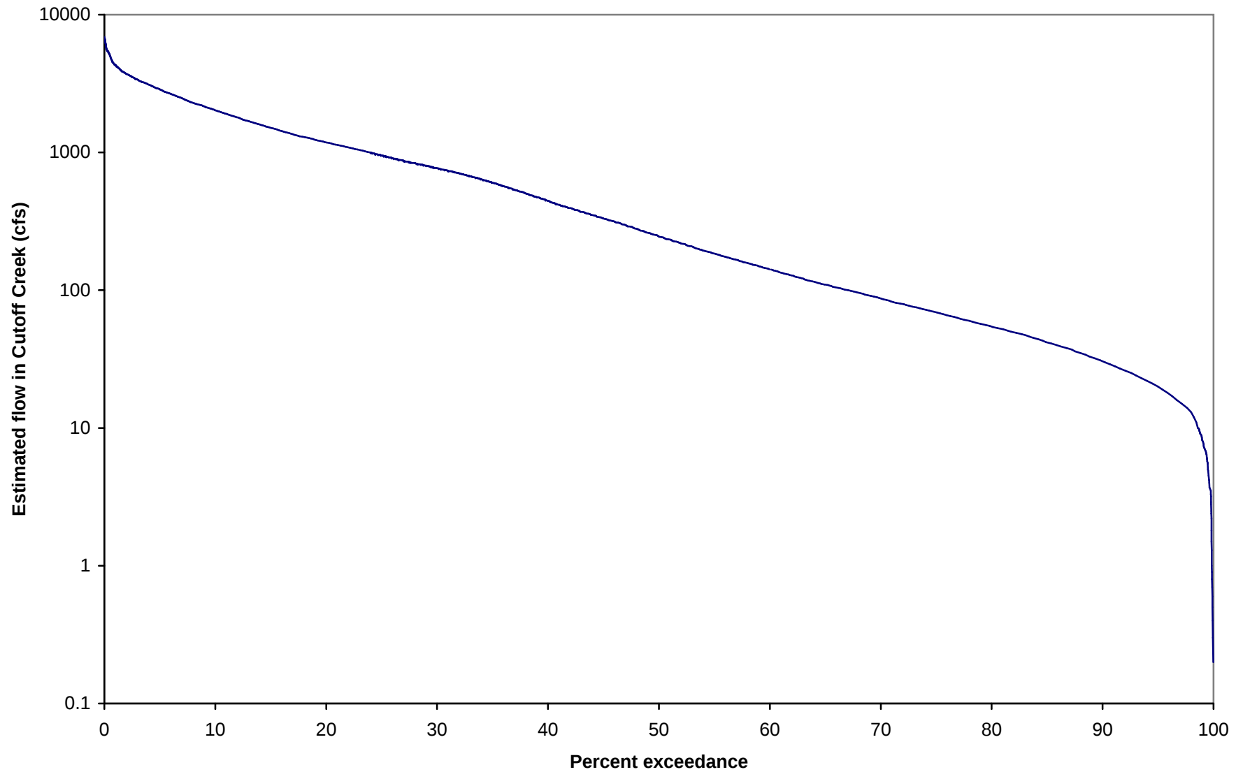
Figure J.1. Flow duration curve for for Cutoff Creek 08040205-007
