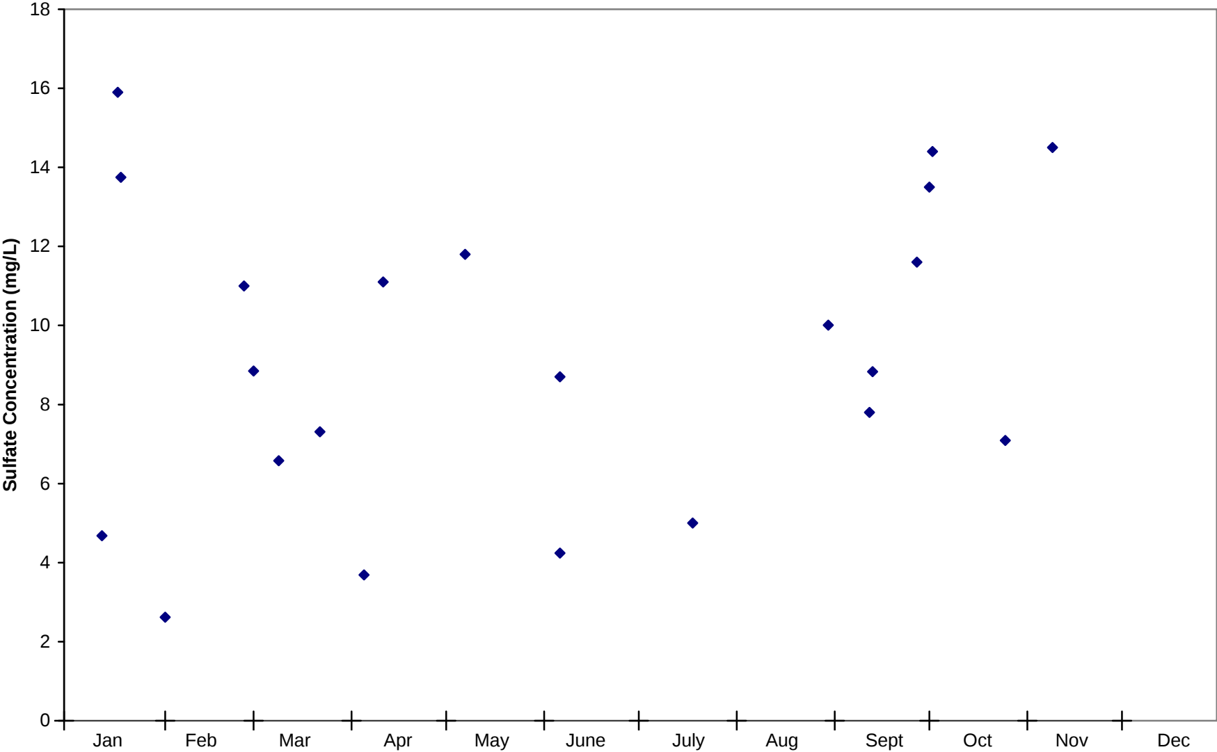
Figure C.5. Seasonal Plot of Sulfate in Bayou Bartholomew near McGehee (UWBYB02)
