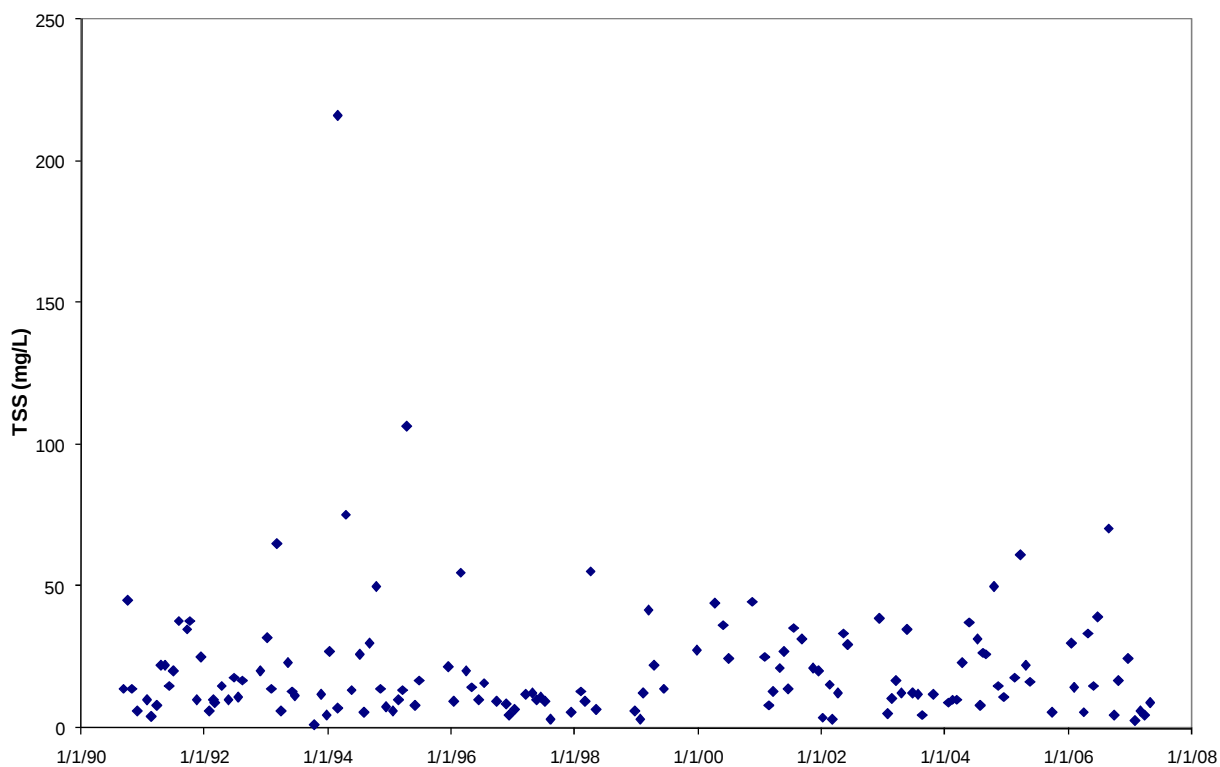
Figure C-3. Time series TSS observations at Big Creek below Sheridan, Arkansas (station OUA0018).
