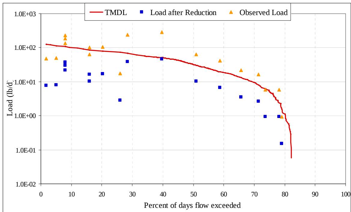
Figure E-1. Base flow TSS load duration curve for station OUA0018 for Big Creek near Sheridan (HUC-reach 08040203-904).
