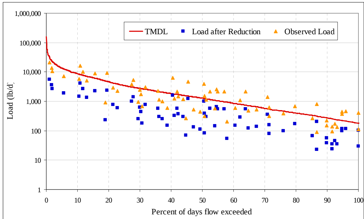
Figure E-2. Storm flow TSS load duration curve for station OUA0018 for Big Creek near Sheridan (HUC-reach 08040203-904).
